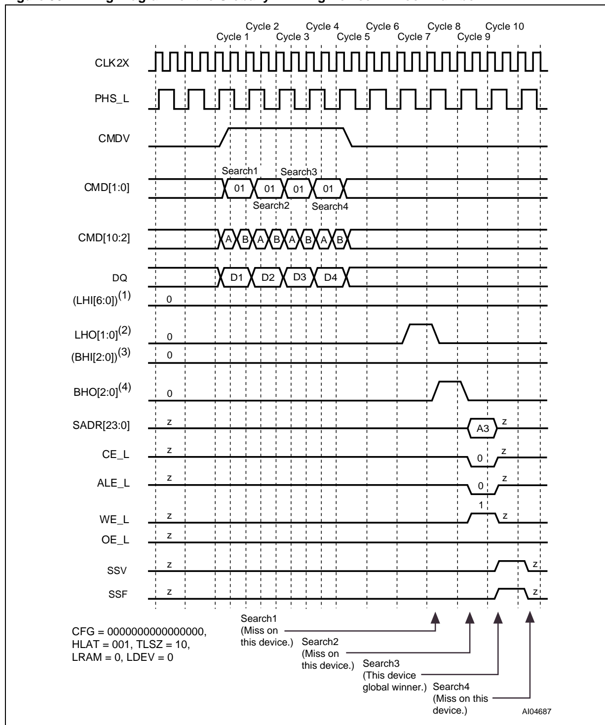
Figure 35. Timing Diagram for the Globally Winning Device in Block Number 1
