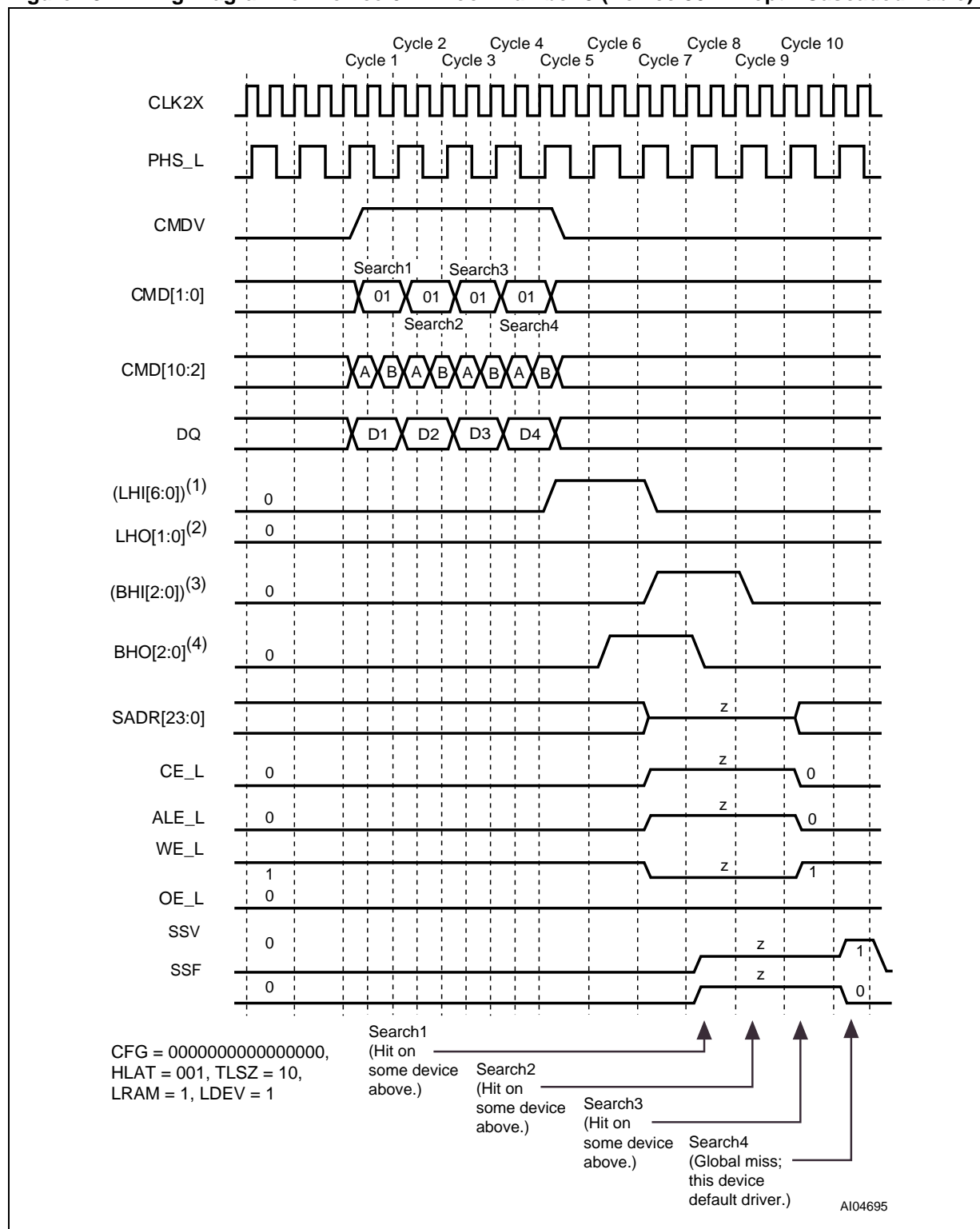
Figure 43. Timing Diagram for Device 6 in Block Number 3 (Device 30 in Depth-Cascaded Table)
