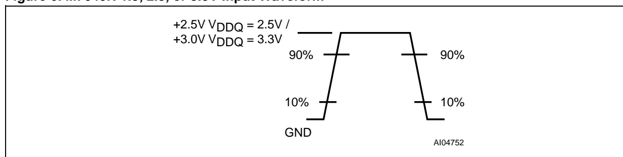
Figure 6. M7040N 1.8, 2.5, or 3.3V Input Waveform
