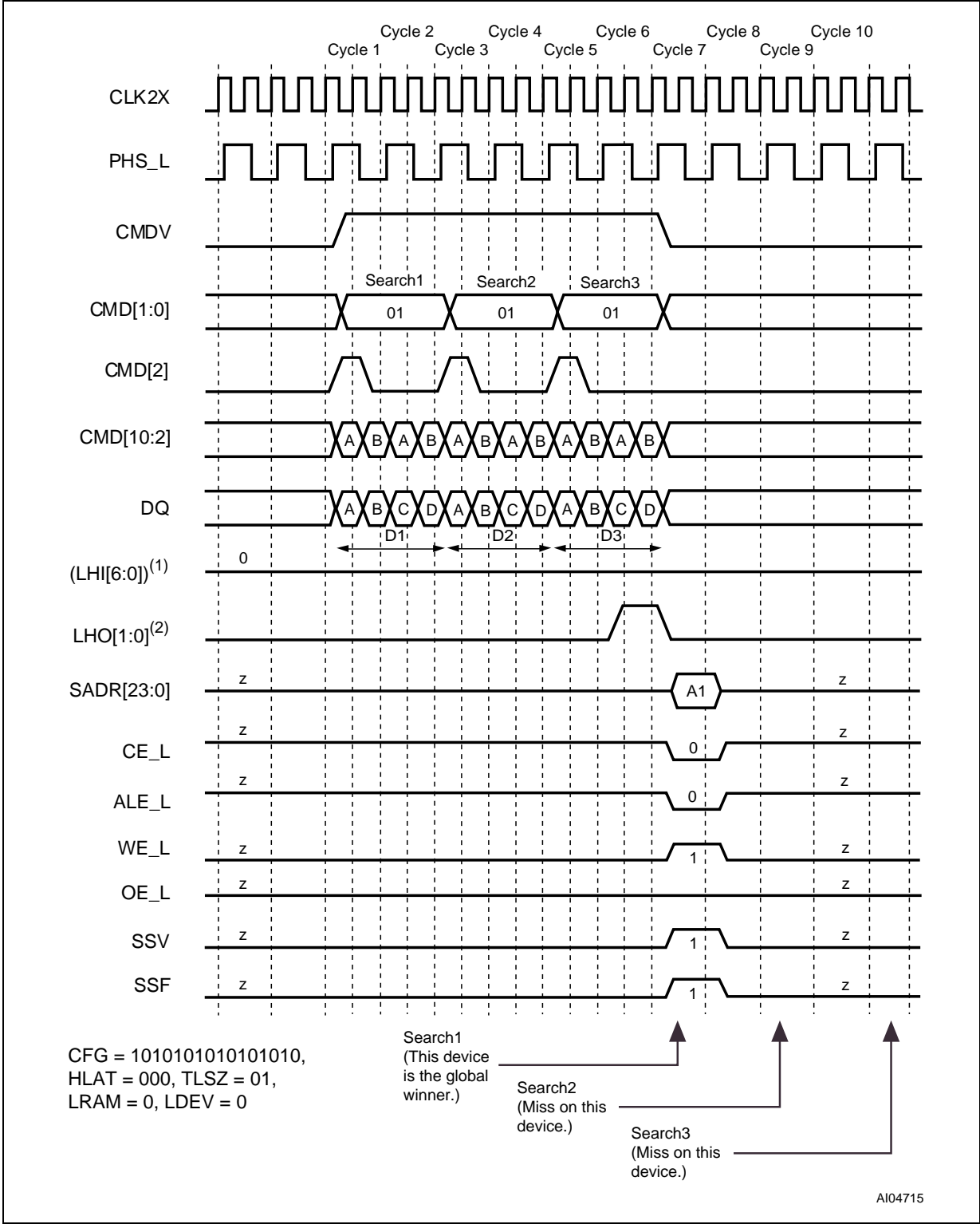
Figure 71. Timing Diagram for 288-bit SEARCH for Device Number 0
