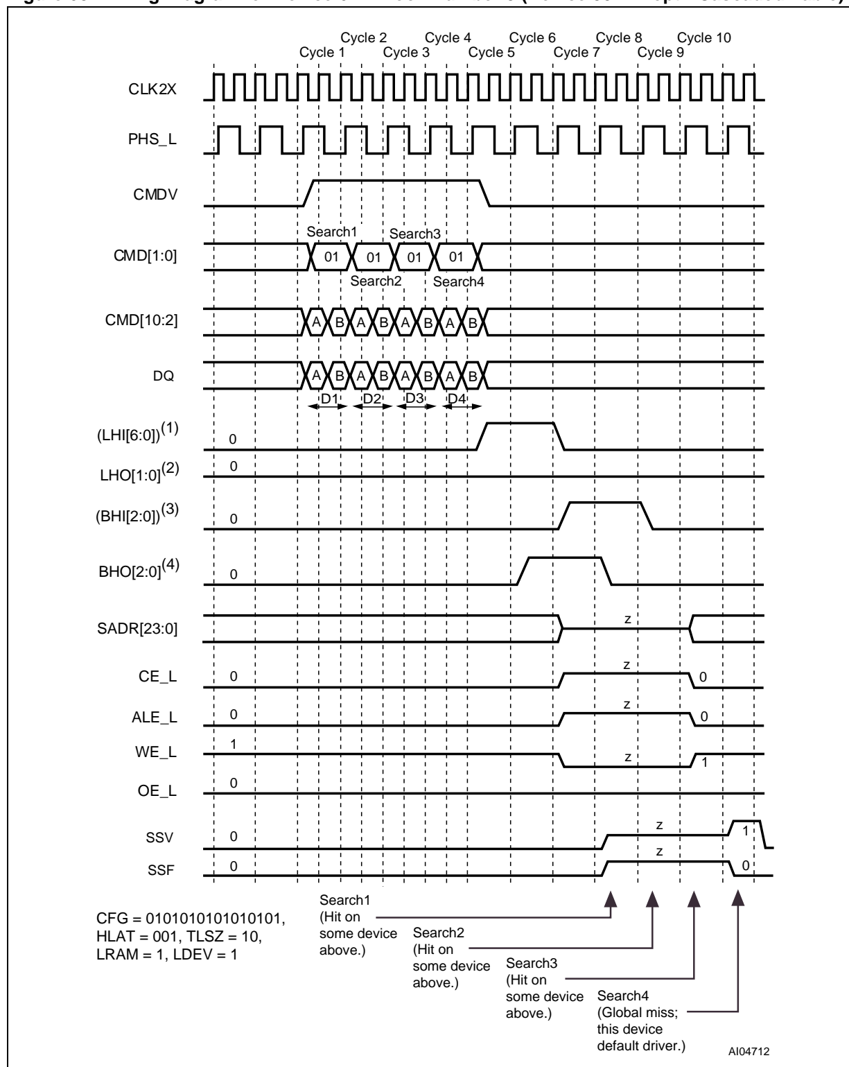
Figure 65. Timing Diagram for Device 6 in Block Number 3 (Device 30 in Depth-Cascaded Table)
