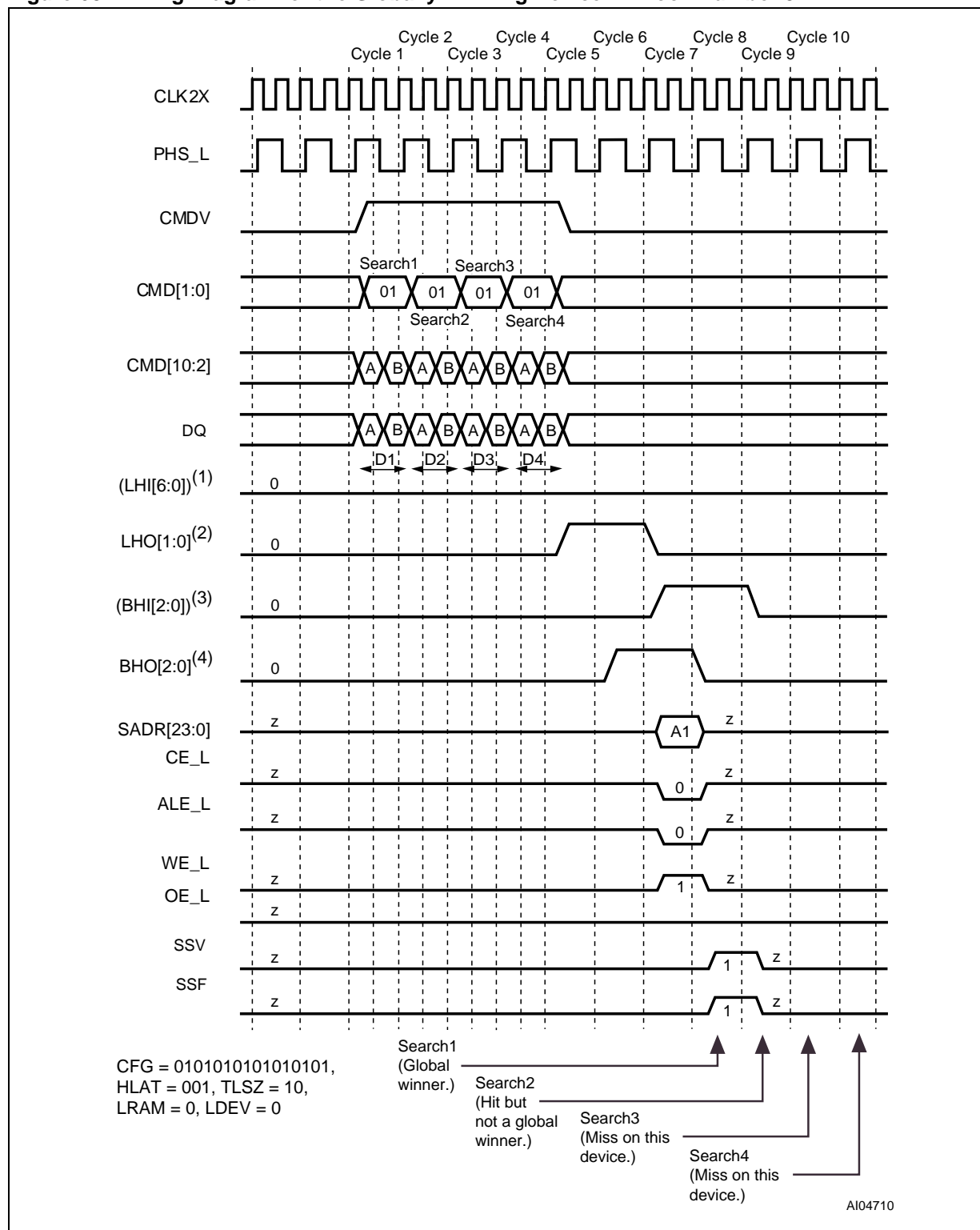
Figure 63. Timing Diagram for the Globally Winning Device in Block Number 3
