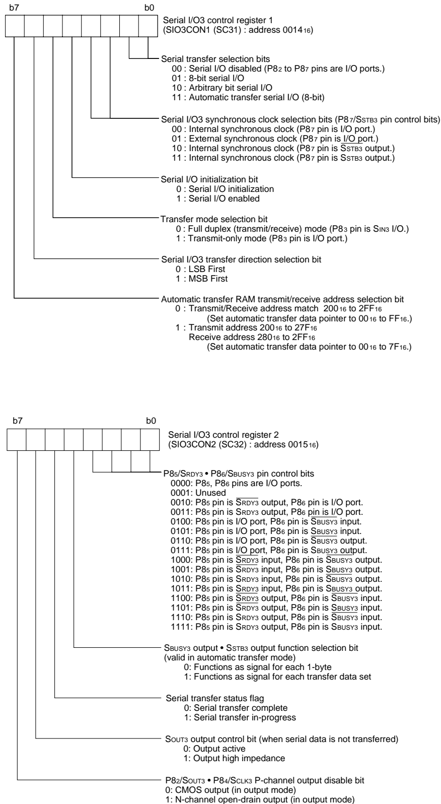
Fig. 35 Structure of serial I/O3 control registers 1 and 2
