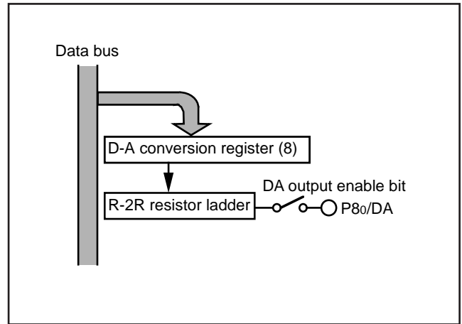
Fig. 61 Block diagram of D-A converter
