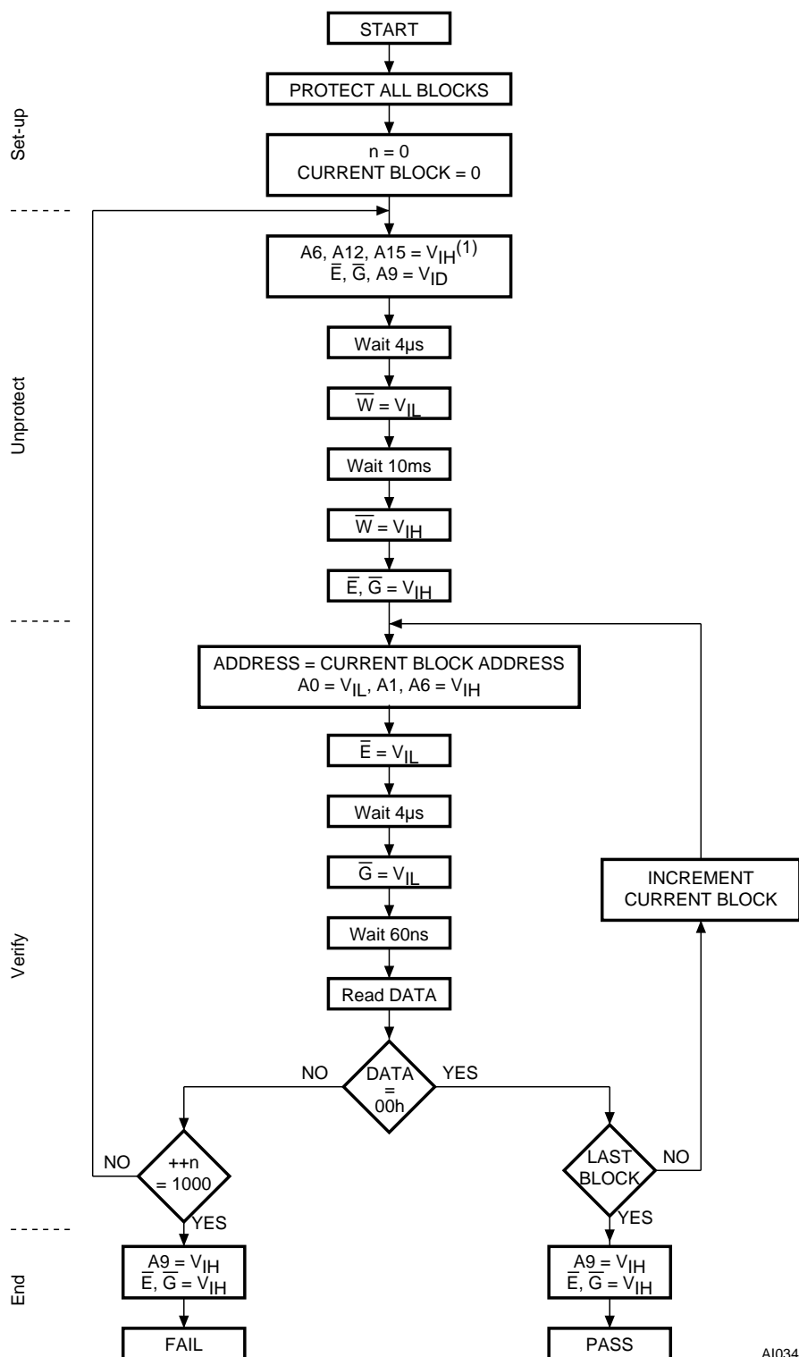
Figure 22. Programmer Equipment Chip Unprotect Flowchart
