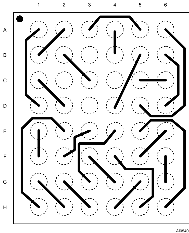
Figure 19. TFBGA48 Daisy Chain - Package Connections (Top view through package)
