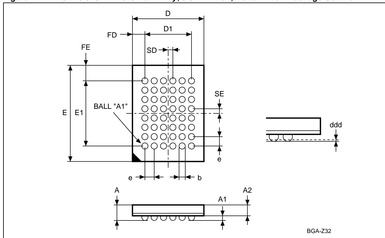
Figure 21. TFBGA48 6x8mm - 6x8 Ball Array, 0.8mm Pitch, Bottom View Package Outline
