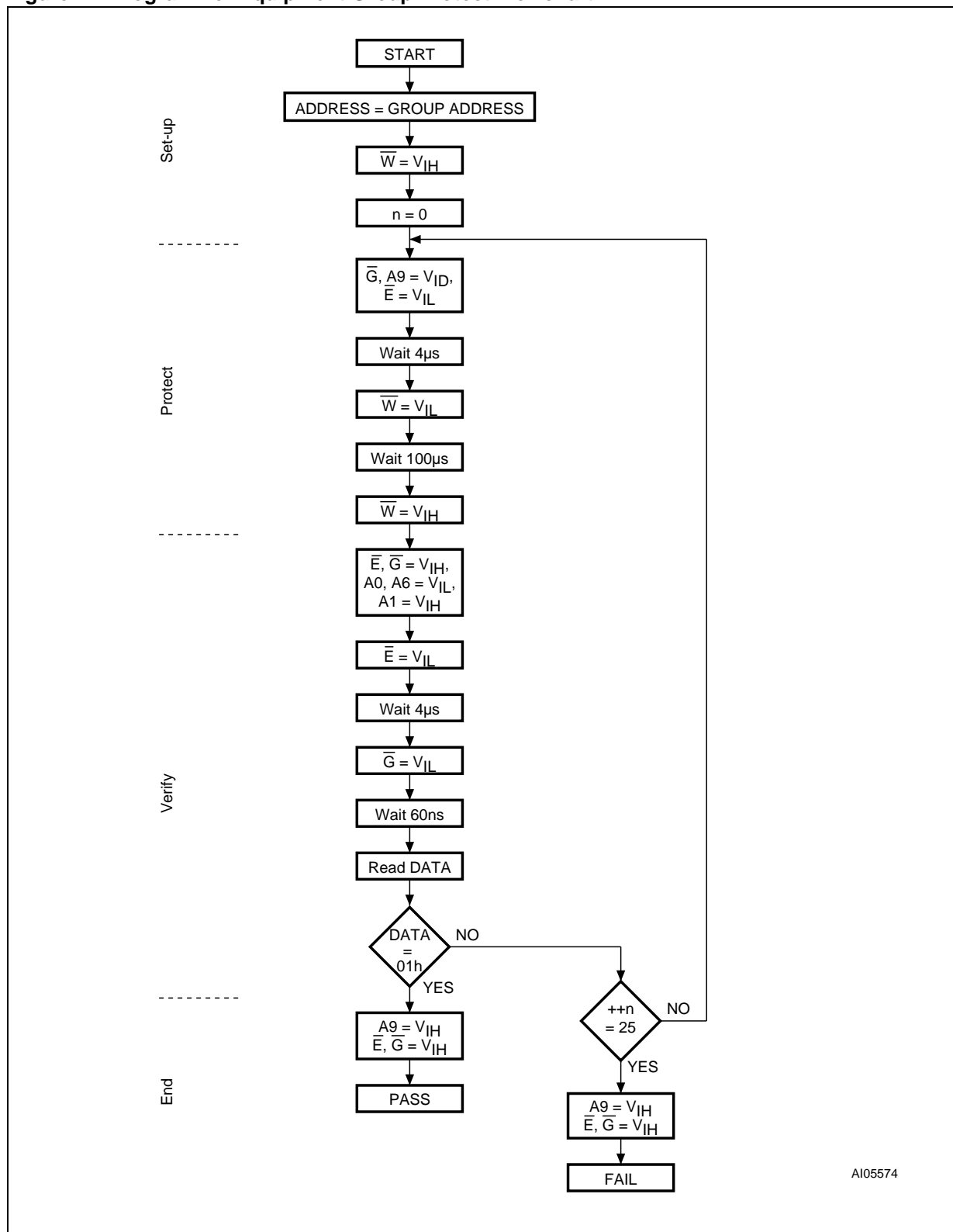
Figure 22. Programmer Equipment Group Protect Flowchart
