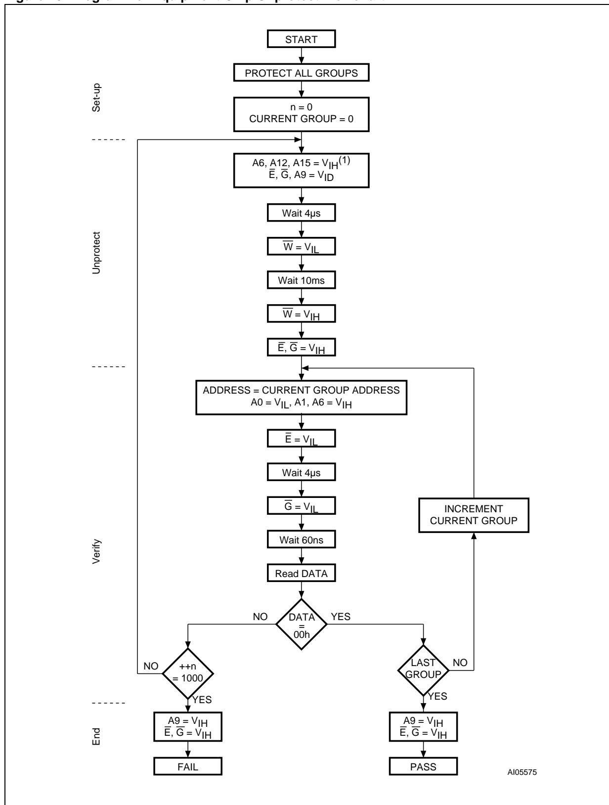
Figure 23. Programmer Equipment Chip Unprotect Flowchart
