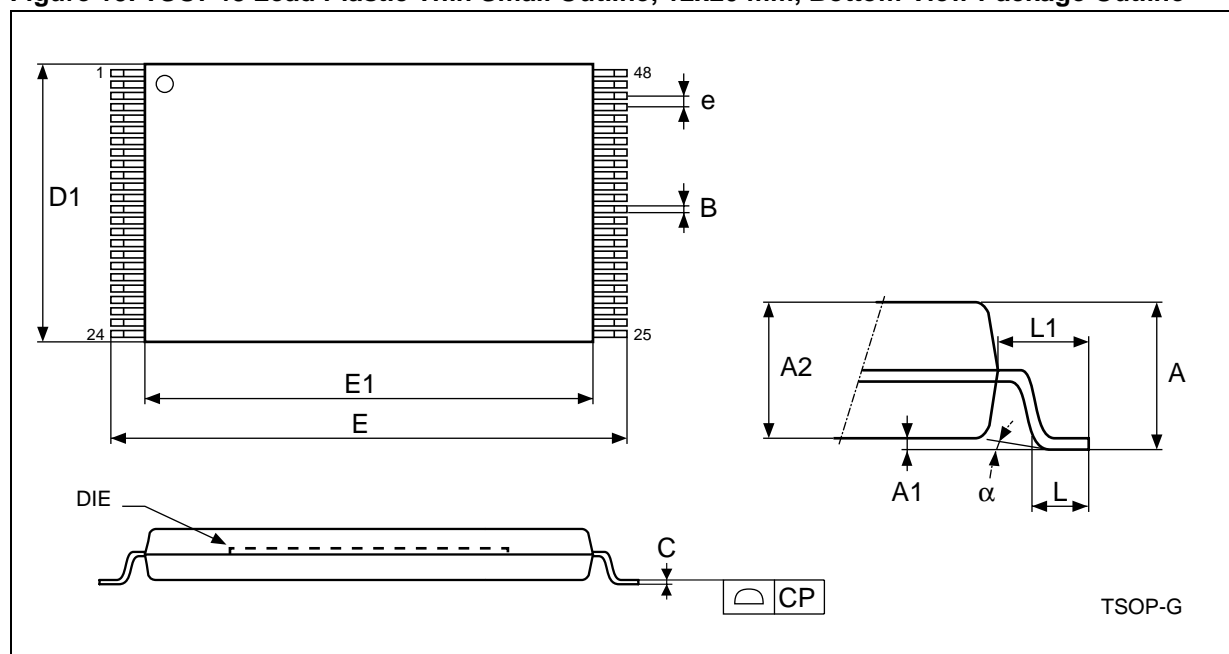
Figure 19. TSOP48 Lead Plastic Thin Small Outline, 12x20 mm, Bottom View Package Outline
