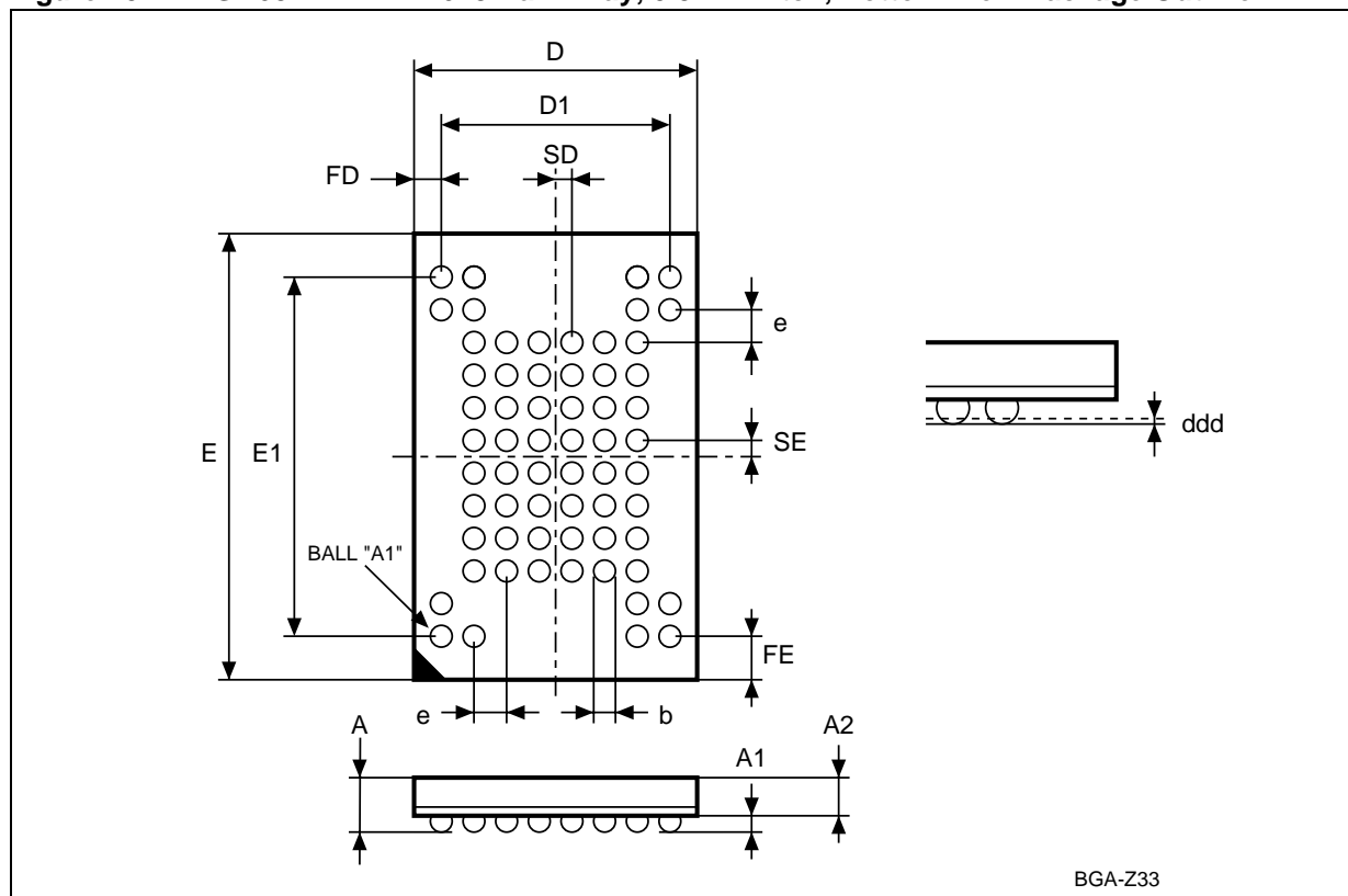
Figure 20. TFBGA63 7x11mm - 6x8 Ball Array, 0.8mm Pitch, Bottom View Package Outline
