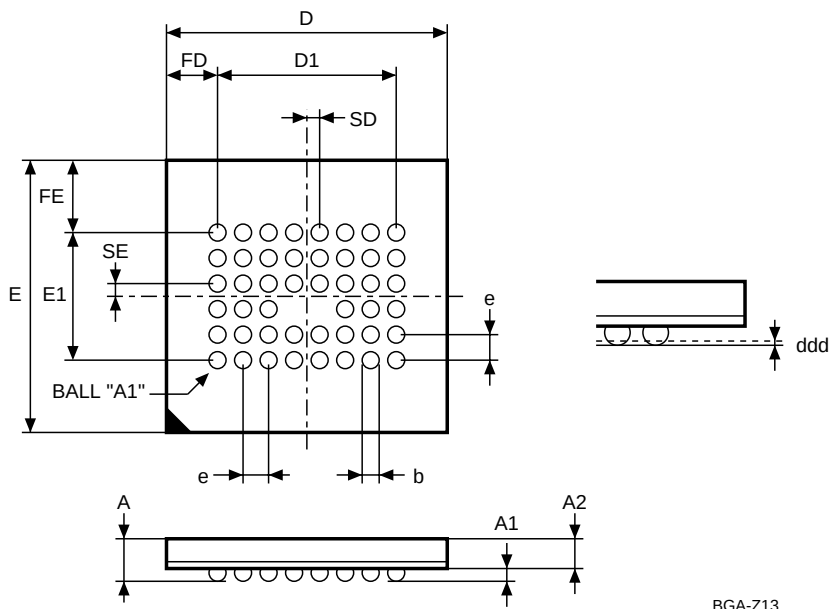
Figure 12. TFBGA46 6.39x6.37mm - 8x6 ball array, 0.75 mm pitch, Bottom View Package Outline
