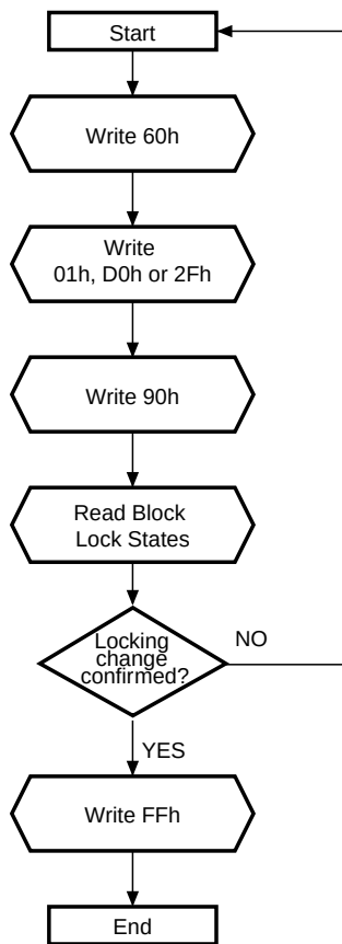
Figure 20. Locking Operations Flowchart and Pseudo Code
