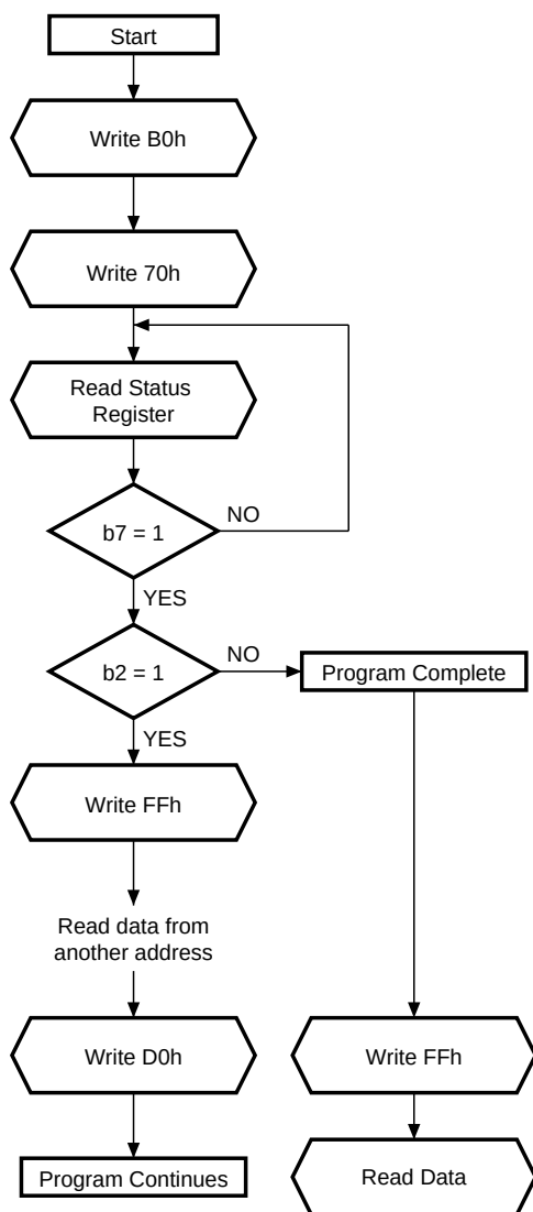
Figure 17. Program Suspend &amp; Resume Flowchart and Pseudo Code
