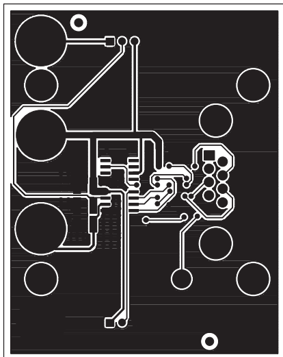
Component Side
