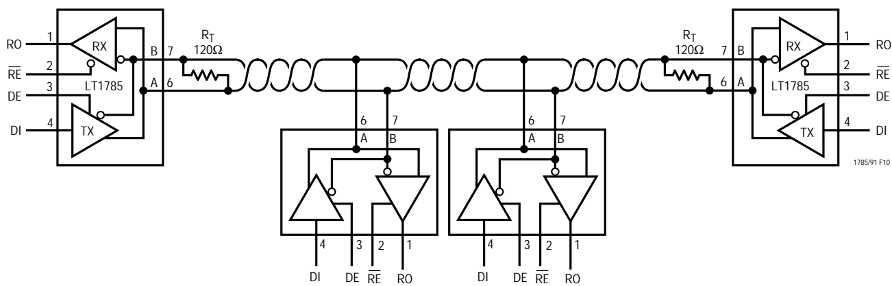
Figure 10. Half-Duplex RS485 Network Operation
