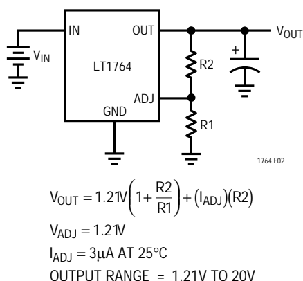
Figure 2. Adjustable Operation
