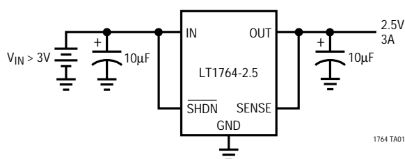
3.3V IN to 2.5V OUT Regulator
