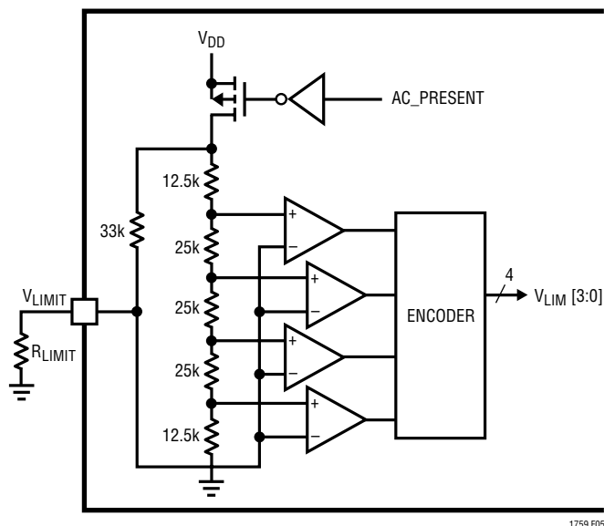
Figure 5. Simplified V_{LIMIT} Circuit Concept ( I_{LIMIT} Is Similar)
