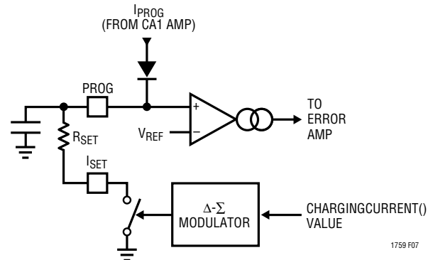
Figure 7. Current DAC Operation
