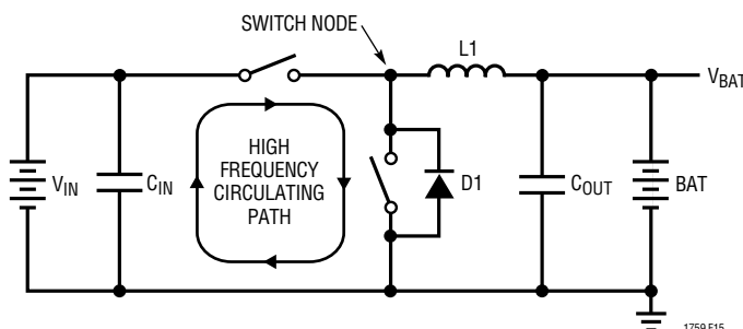
Figure 15. High Speed Switching Path
