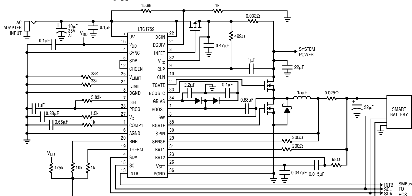
Figure 1. 4A SMBus Smart Battery Charger
