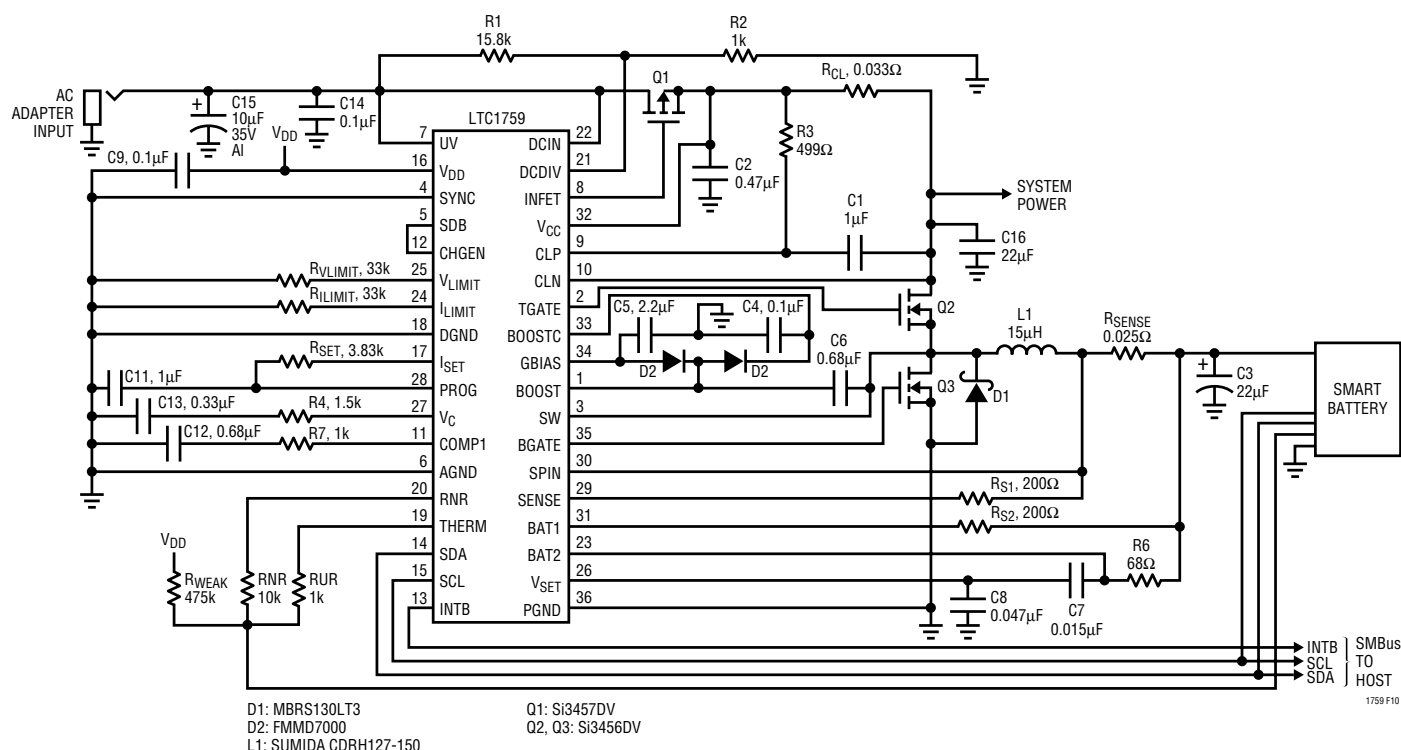
Figure 10. 4A SMBus Smart Battery Charger
