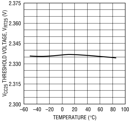
V CC25 Threshold Voltage vs Temperature
