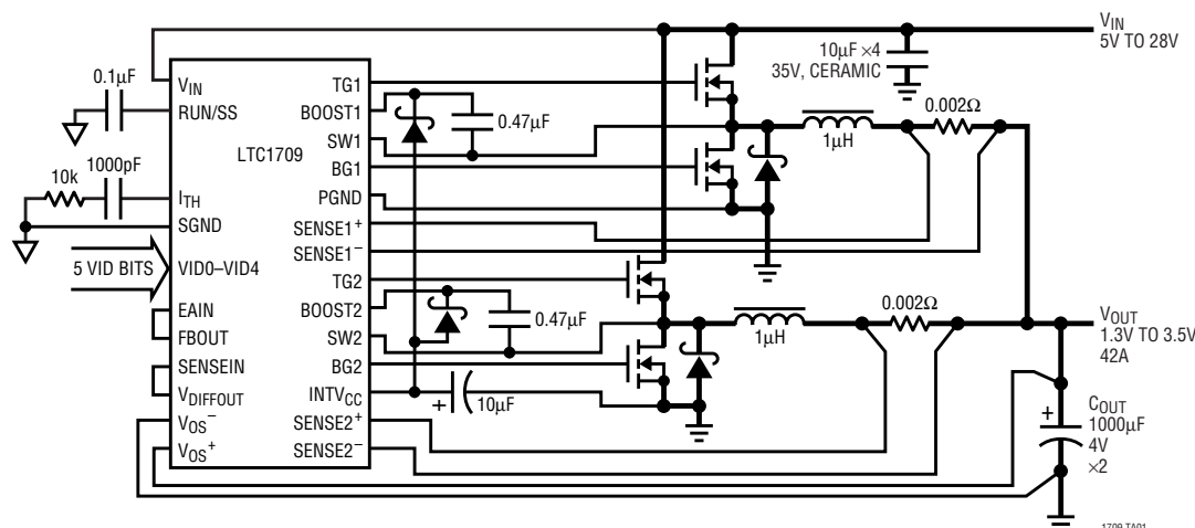
Figure 1. Surface Mount, 42A, 2-Phase Step-Down Converter
