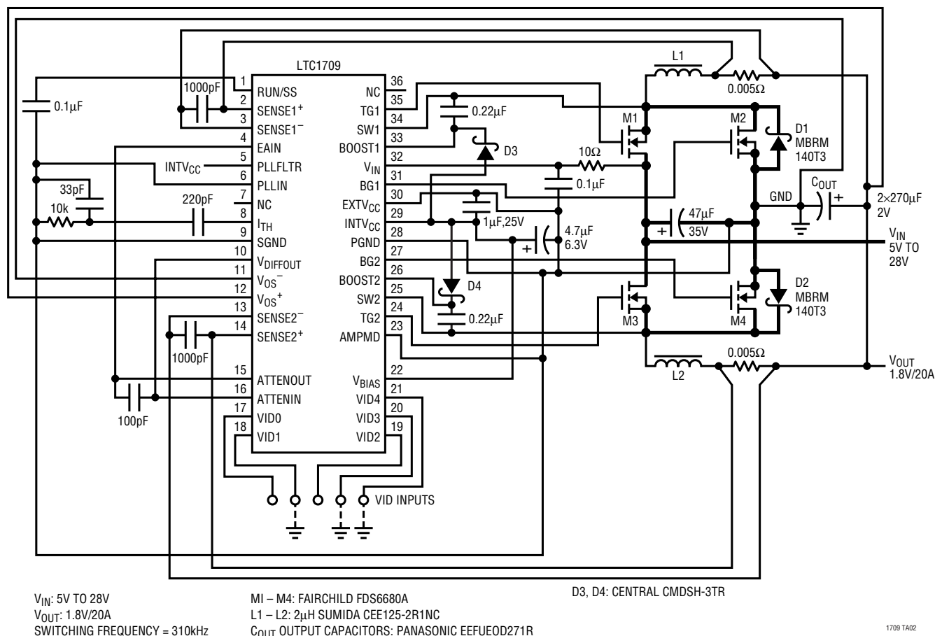
Figure 11. 5V Input, 1.8V/20A Power Supply
