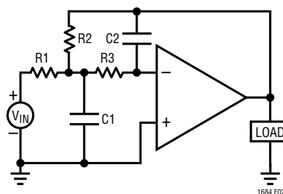
Figure 2a. Lowpass Infinite-Gain Multiple Feedback Filter
