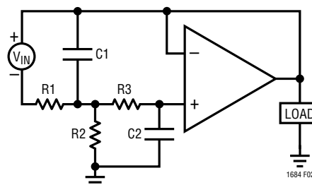
Figure 2b. Active Tracking Supply Transformed Multiple Feedback Filter
