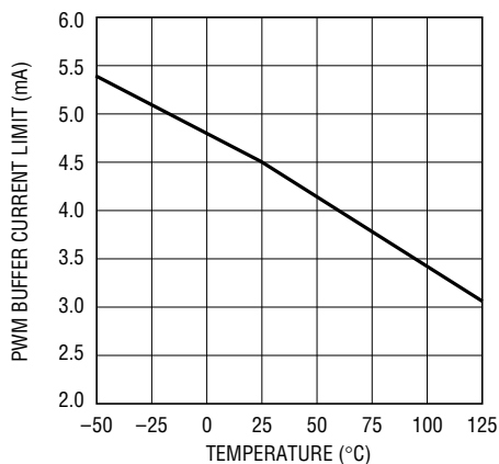
PWM Buffer (Pin \text{BG}_{\text{OUT}} ) Current Limit vs Temperature
