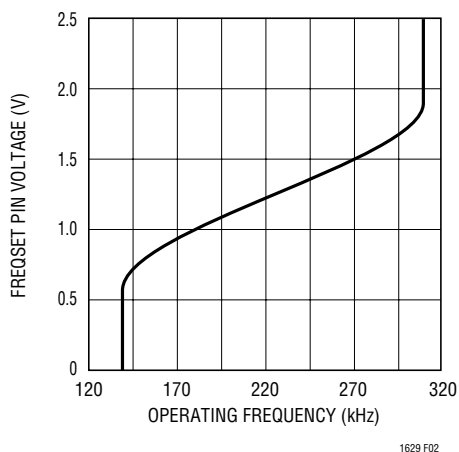
Figure 2. Operating Frequency vs V_{\text{PLLFLTR}}
