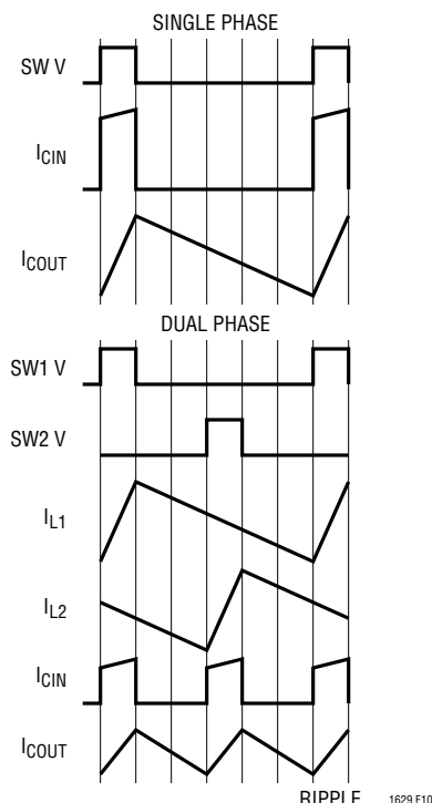
Figure 10. Single and PolyPhase Current Waveforms
