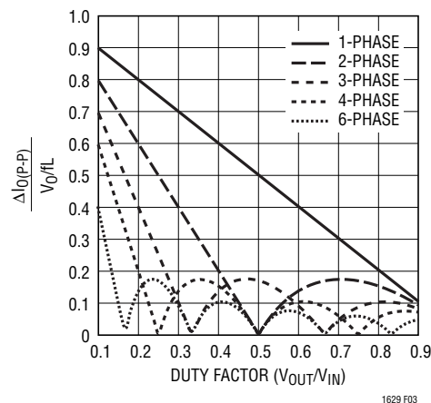
Figure 3. Normalized Peak Output Current vs Duty Factor [ I_{\text{RMS}} \approx 0.3 (\Delta I_{\text{O(P-P)}) ]
