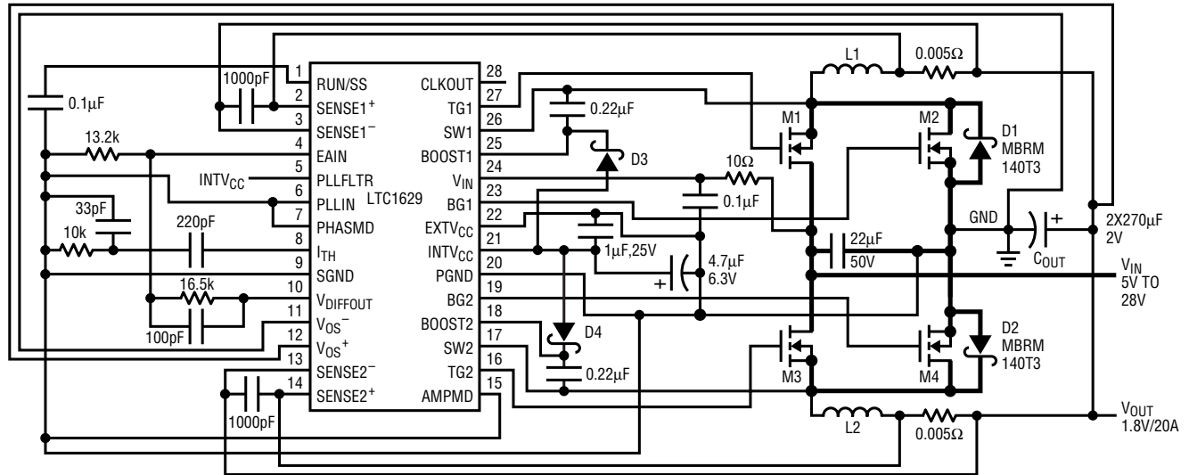
1.8V/20A CPU Power Supply
