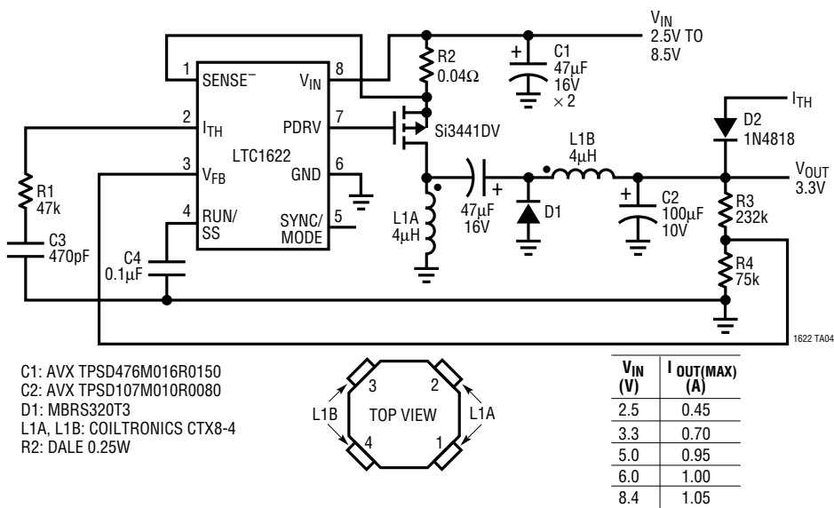
Zeta Converter with Foldback Current Circuit
