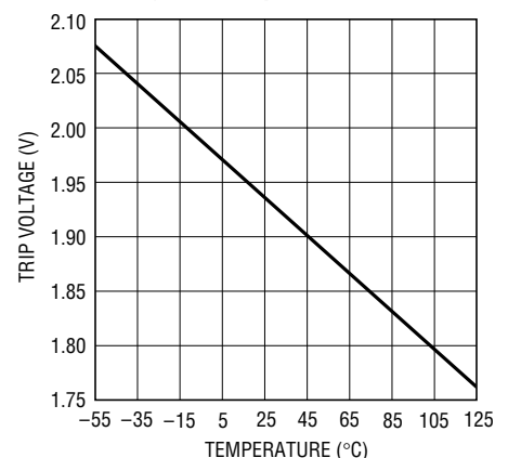
Undervoltage Lockout Trip Voltage vs Temperature
