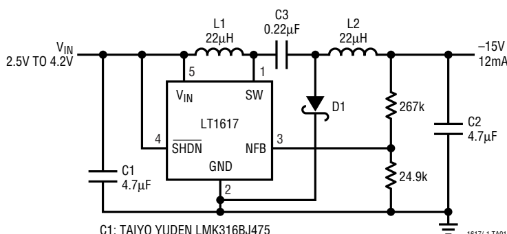
1-Cell Li-Ion to -15V Inverting Converter
