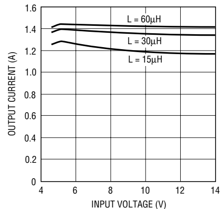
Maximum Output Current at V_{OUT} = 2.5V
