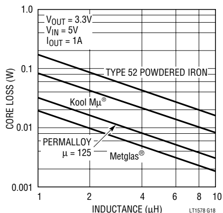
Inductor Core Loss
