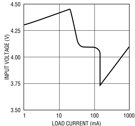
Minimum Input Voltage to Start with 3.3V Output
