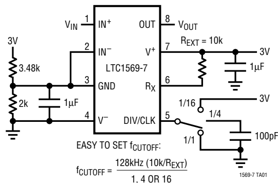
Single 3V Supply, 128kHz/32kHz/8kHz Lowpass Filter
