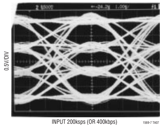
4-Level Eye Diagram
