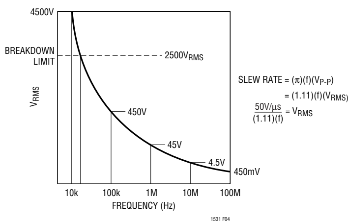
Figure 4. V_{RMS} vs Frequency
