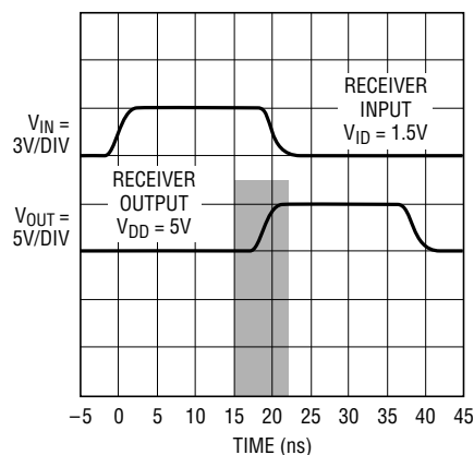
Propagation Delay Guaranteed to Fall Within Shaded Area ( \pm 3.5\text{ns} )
