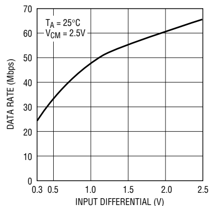
Maximum Data Rate vs Input Differential Voltage
