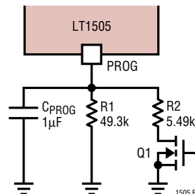
Figure 7. 2-Level Charging
