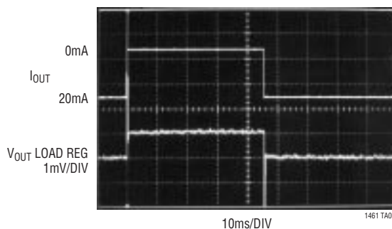
Load Regulation, P DISS = 200mW
