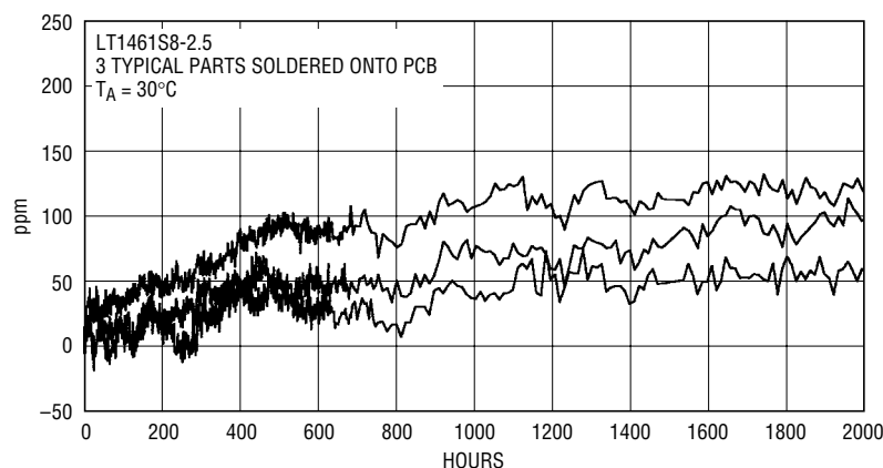
Long-Term Drift
