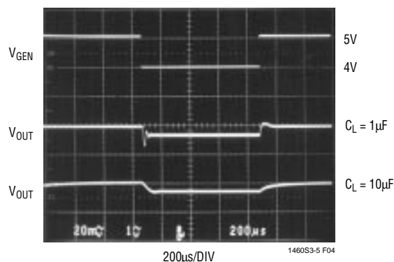
Figure 4. I_{OUT} = 1mA
