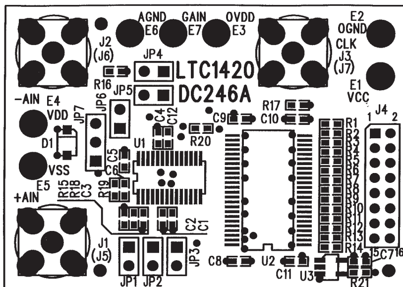
Figure 15. Top Silkscreen Layer for LTC1420 Demo Board
