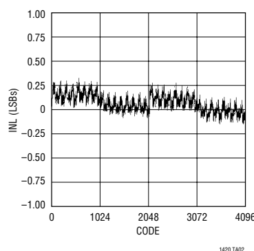
Typical INL Curve
