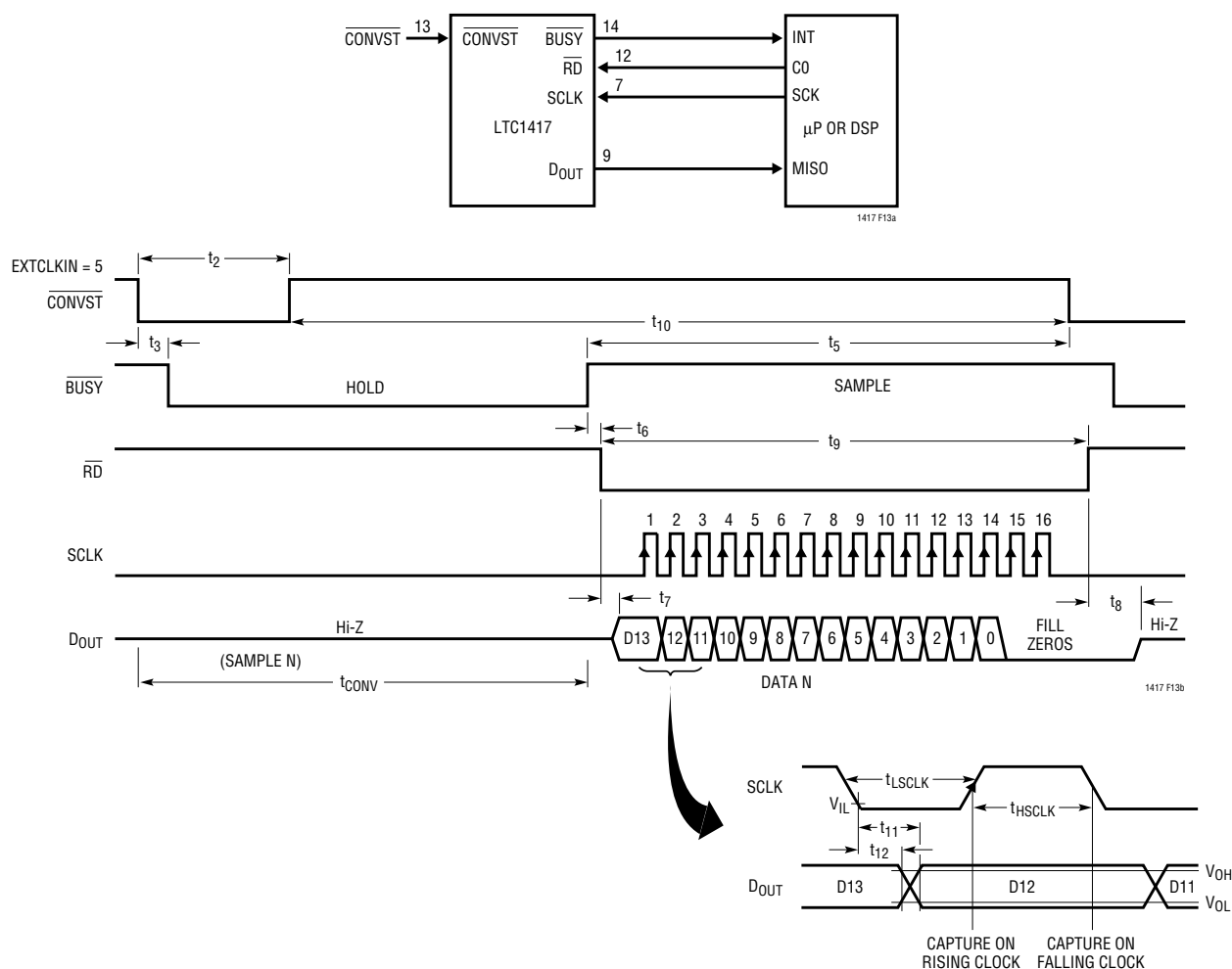
Figure 13. Internal Conversion Clock Selected. Data Transferred After Conversion Using an External SCLK. BUSY\uparrow Indicates End of Conversion
