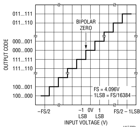
Figure 5b. LTC1417 Bipolar Transfer Characteristics
