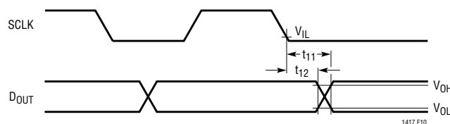
Figure 10. SCLK to D_{OUT} Delay
