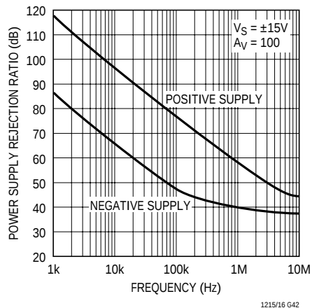
Input Referred Power Supply Rejection Ratio vs Frequency
