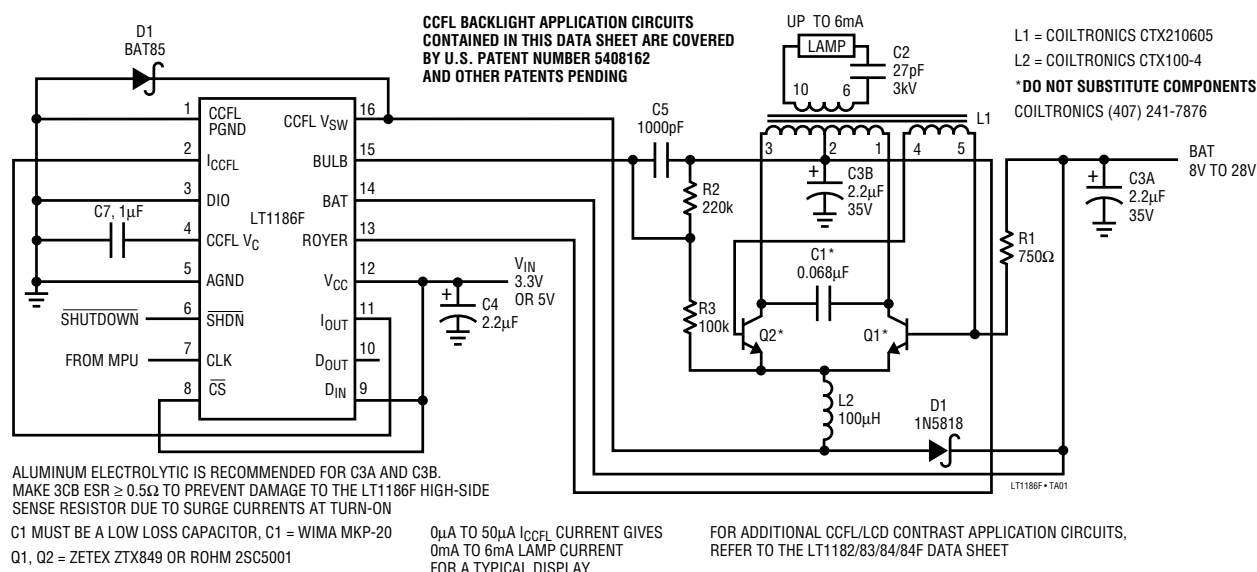
90% Efficient Floating CCFL with 1-Wire (Increment Only) Pulse Mode Control of Lamp Current
