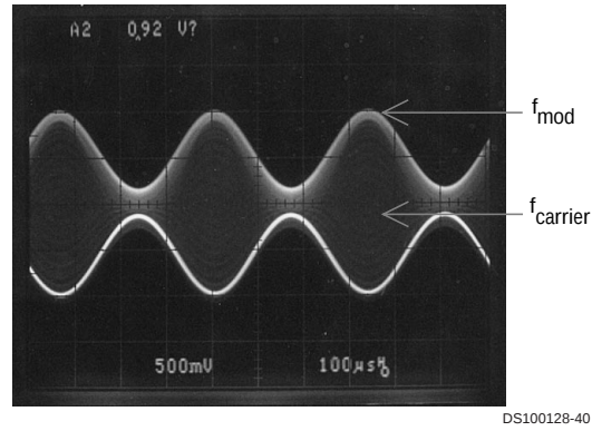
FIGURE 9. Output signal per the Circuit of Figure 8
