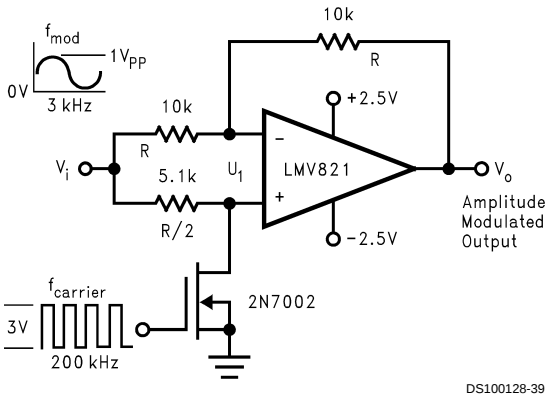
FIGURE 8. Amplitude Modulator Circuit
