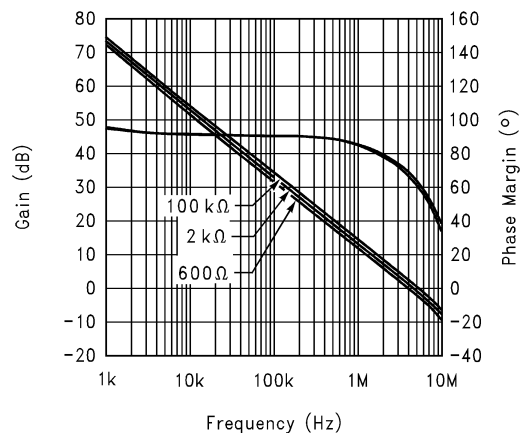
Gain and Phase Margin vs. Frequency (R_L = 100k\Omega, 2k\Omega, 600\Omega) 2.7V
