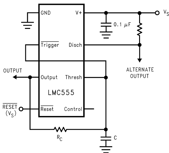
FIGURE 12. 50% Duty Cycle Oscillator
