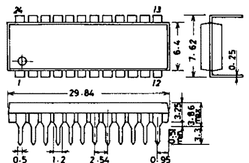
Package Dimensions 3084 (unit: mm)
