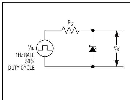
Figure 2. Startup Characteristics Test Circuit
