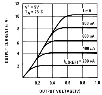
Output Characteristics
