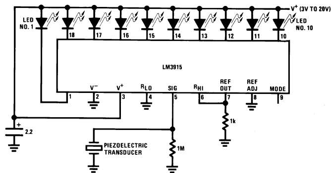
Vibration Meter
