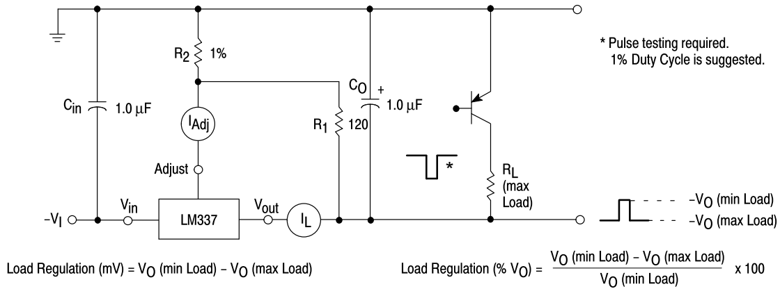
Figure 3. Standard Test Circuit
