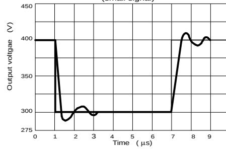
Fig.10 Output Characteristics current sourcing
