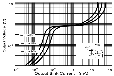
Fig.11 Output Characteristics Current sinking
