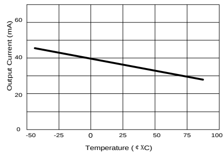
Fig.12 Current Limiting
