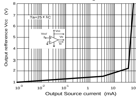
Fig.12 Current Limiting
