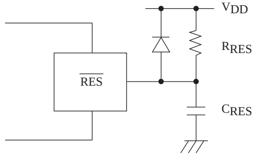
Figure4. Reset circuit
