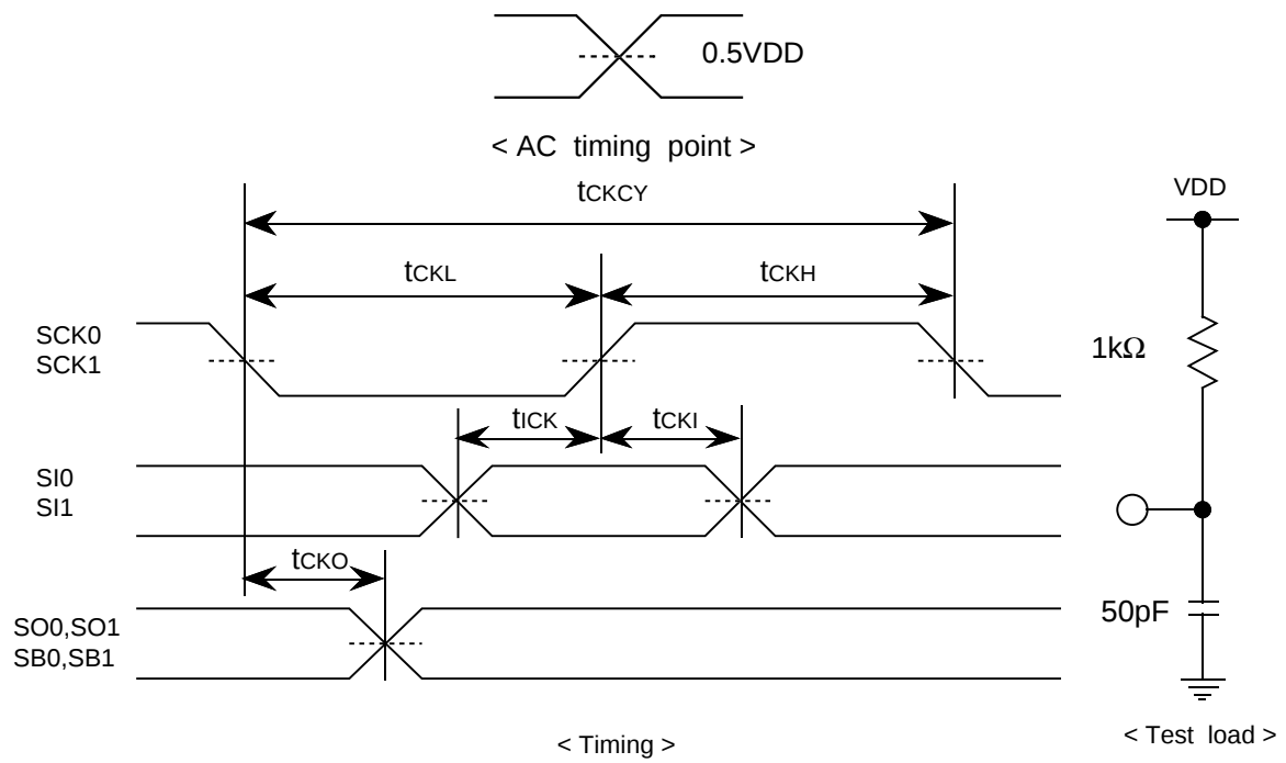
Figure 5 Serial Input/Output Test Conditions
