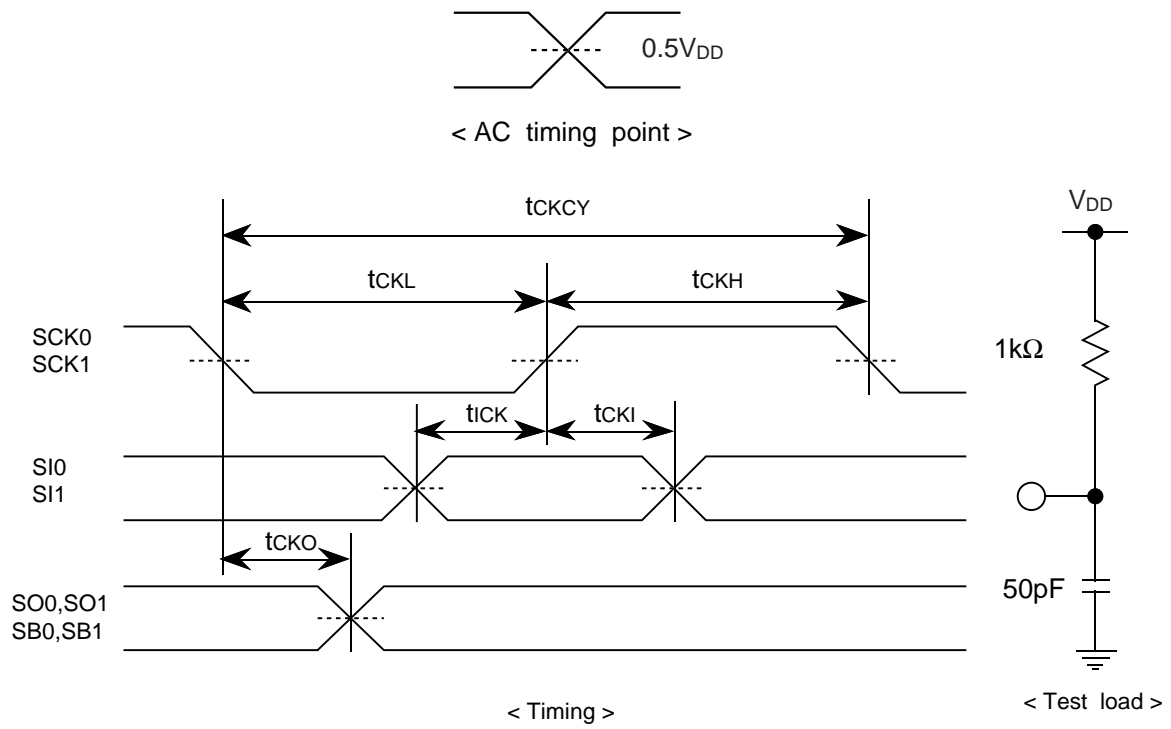
Figure 5 Serial Input/Output Test Conditions
