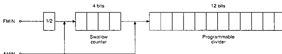
Figure 7. Programmable divider
