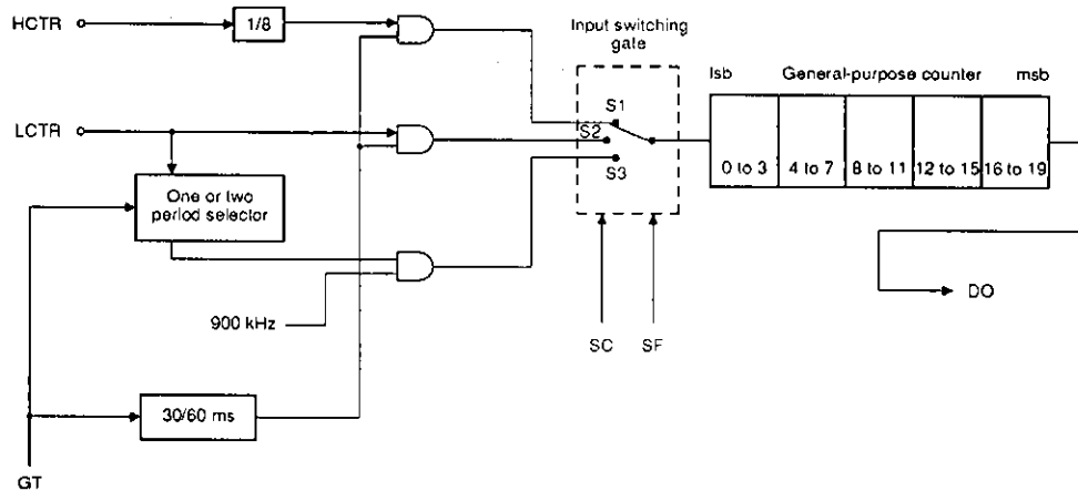
Figure 8. General-purpose counter
