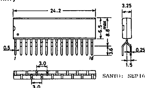
Package Dimensions (unit: mm) 3020A
