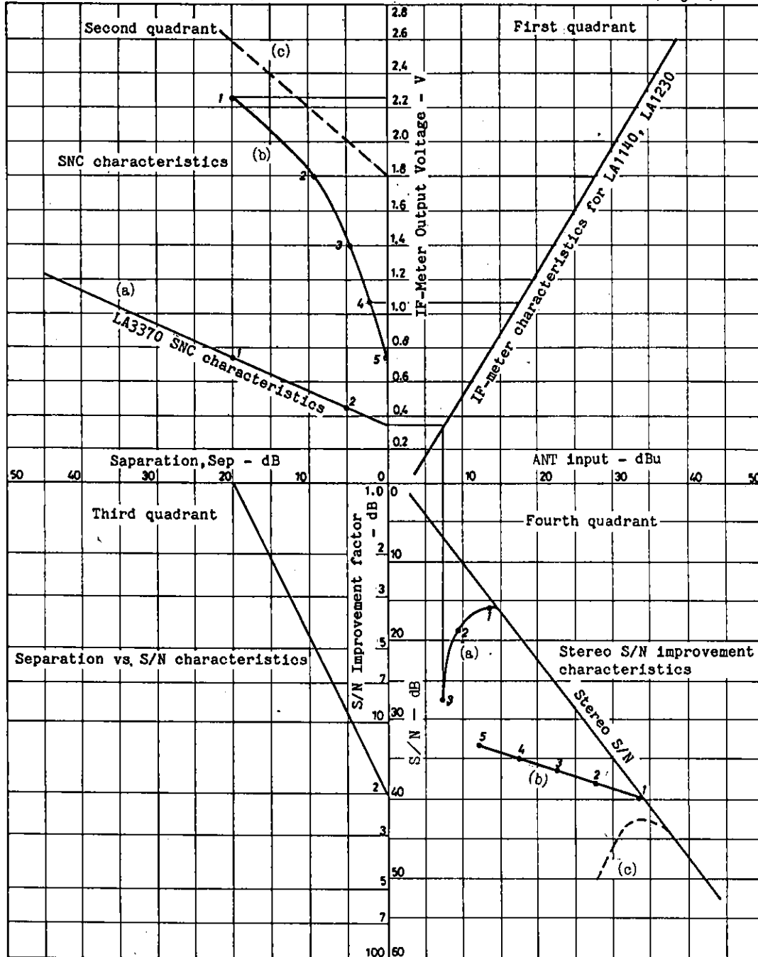
Chart to Obtain Stereo S/N Characteristics from SNC Characteristics (Fig.6)
