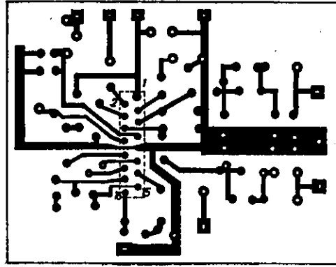
Printed Circuit Pattern
