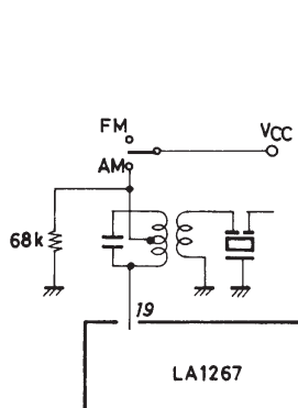
(A) pin 19-use method for AM/FM changeover
