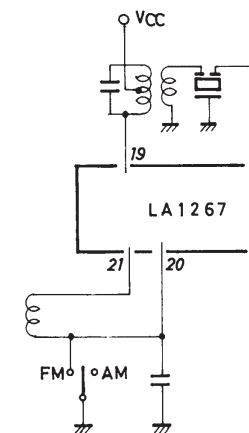
(B) Pin 20-used method for AM/FM changeover
