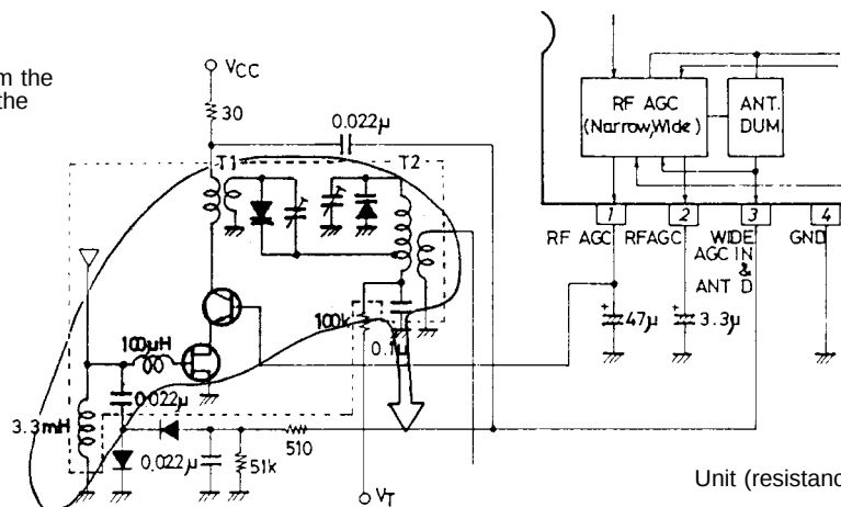
LA1136N/1137N Antenna, RF circuit
