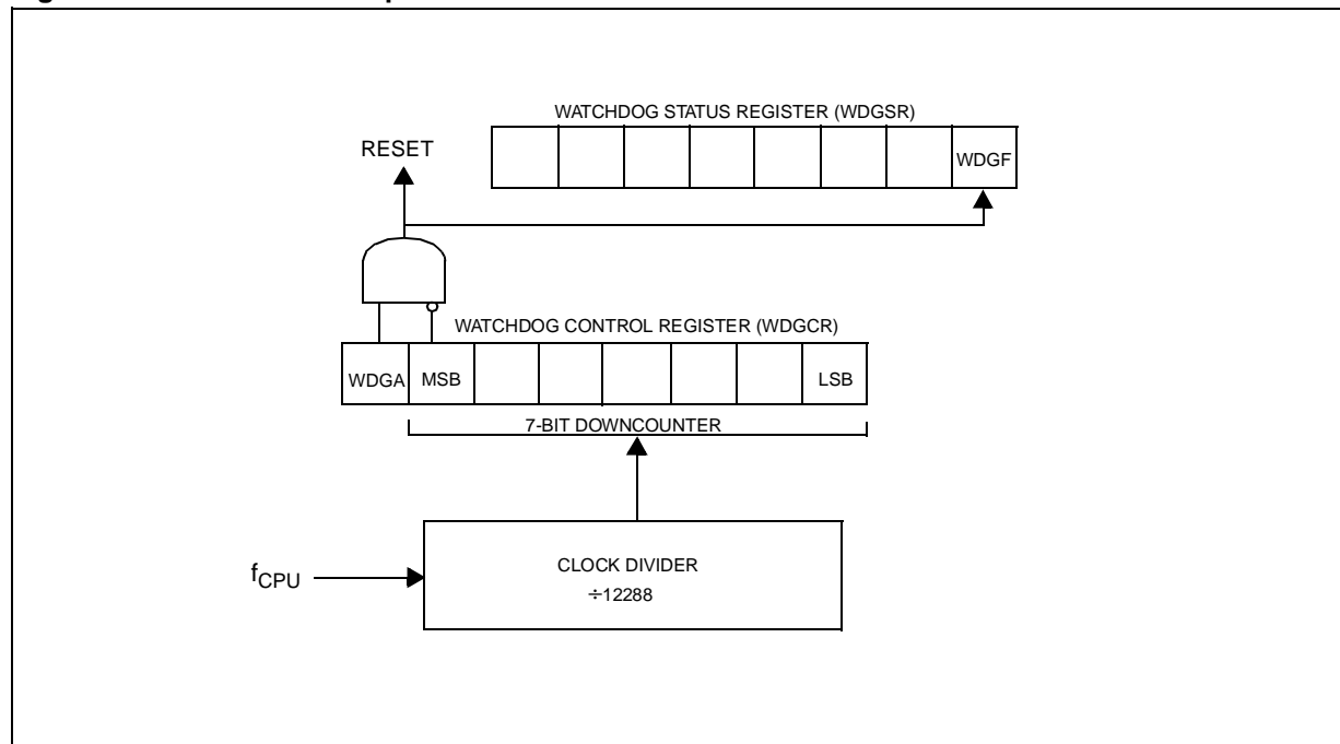
Figure 8. Functional Description
