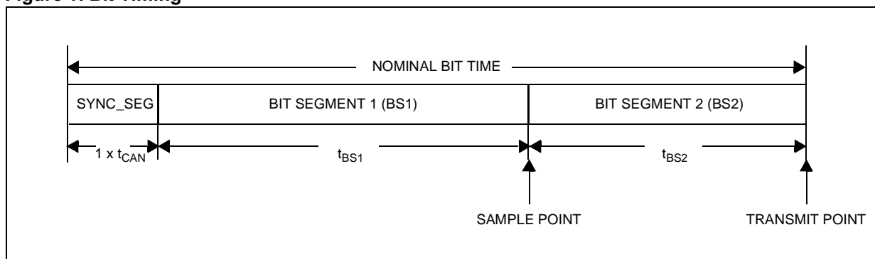
Figure 1. Bit Timing
