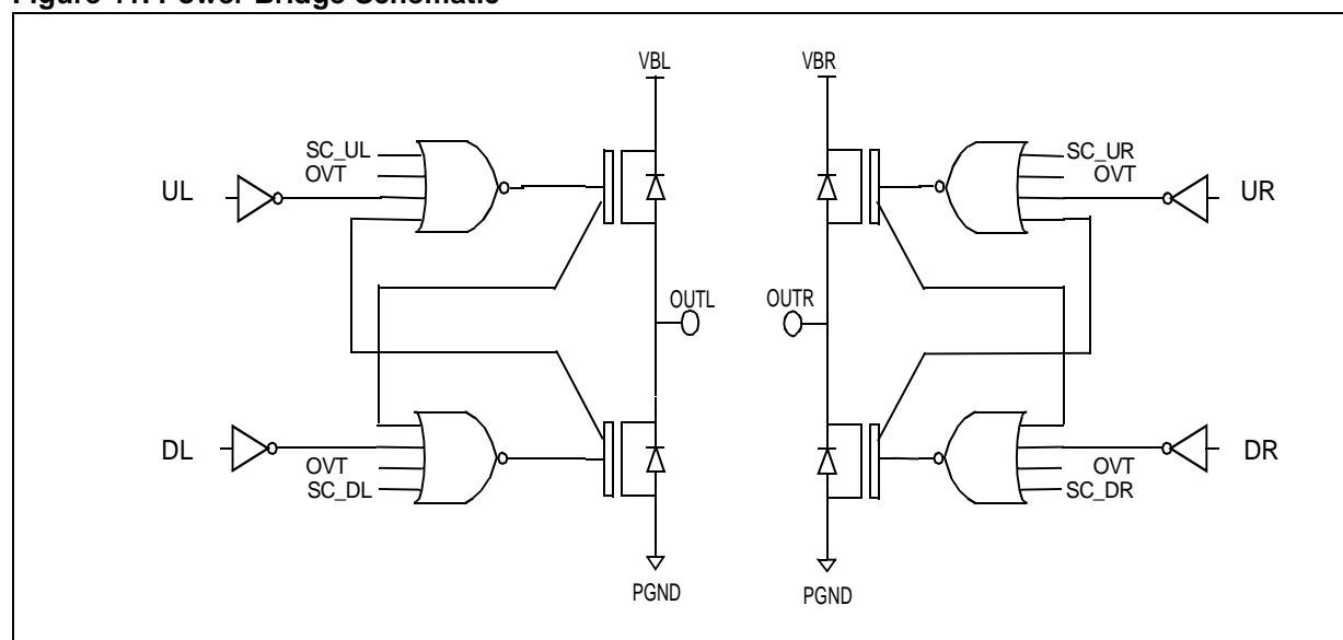
Figure 41. Power Bridge Schematic
