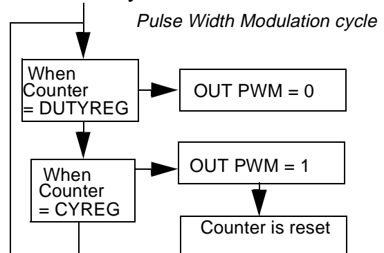
Figure 26. PWM Cycle
