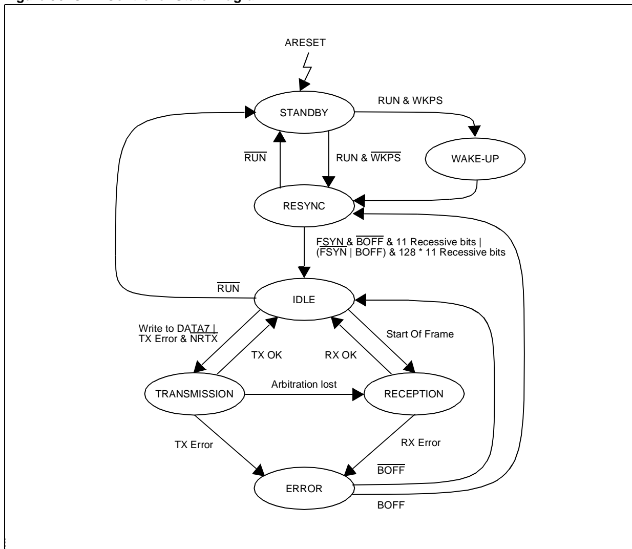
Figure 36. CAN Controller State Diagram
