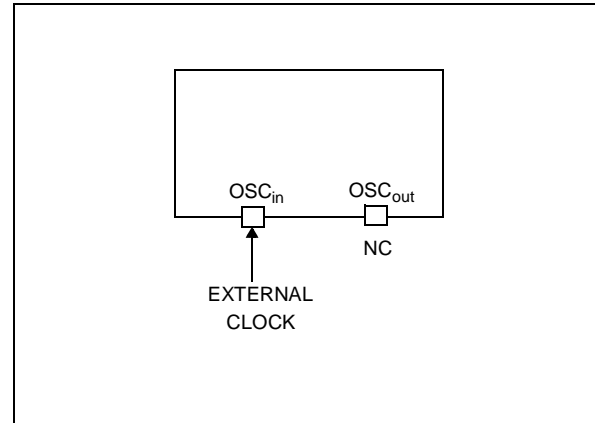
Figure 4. External Clock Source Connections
