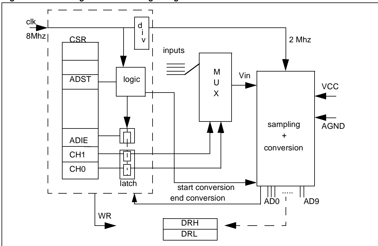
Figure 32. Block diagram of the Analog to Digital Converter
