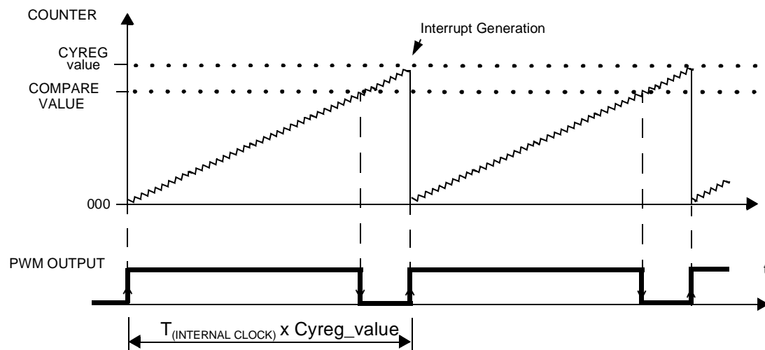
Figure 27. PWM Generation
