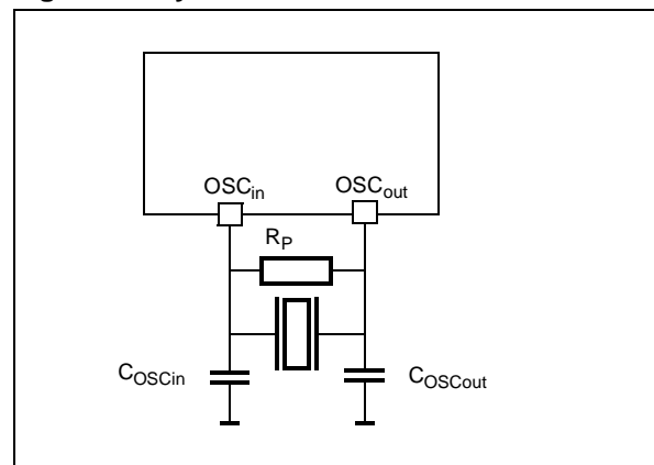
Figure 5. Crystal/Ceramic Resonator
