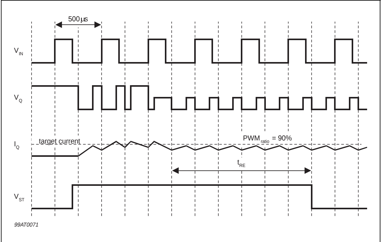
Figure 15. Overtemperature
