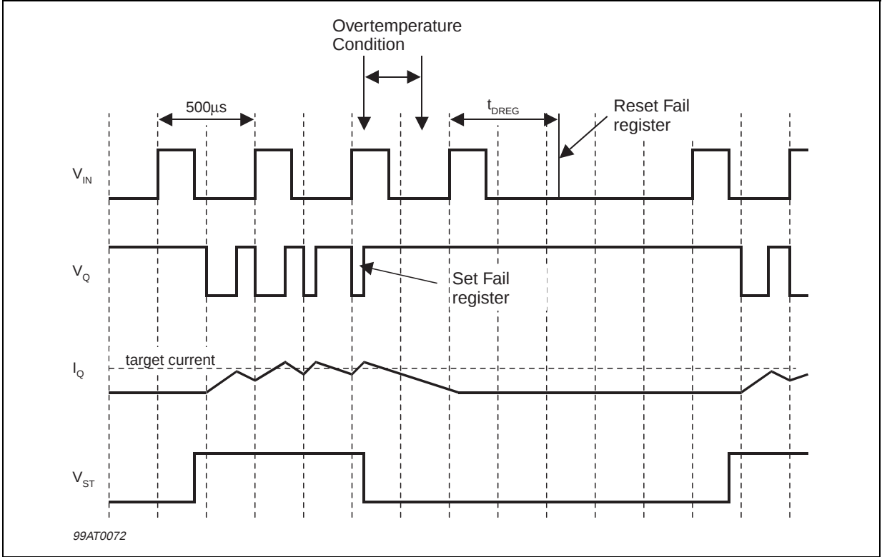
Figure 15. Overtemperature
