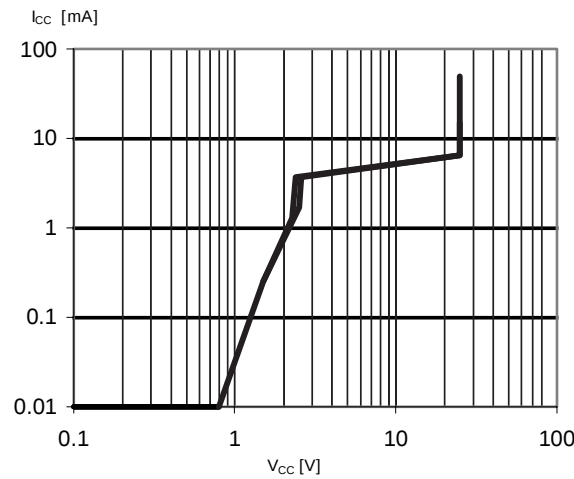
Figure 3. Supply current
