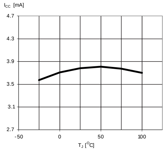
Figure 3. Supply current
