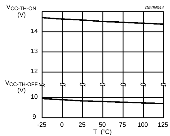
Figure 7: Undervoltage Lockout Threshold vs. Temperature
