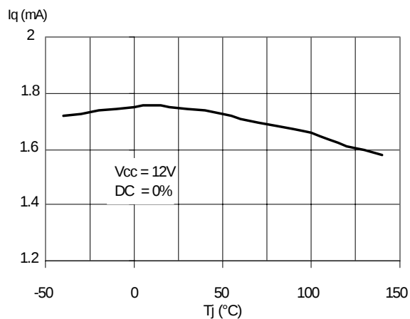
Figure 5. Shutdown Current vs. Junction Temperature
