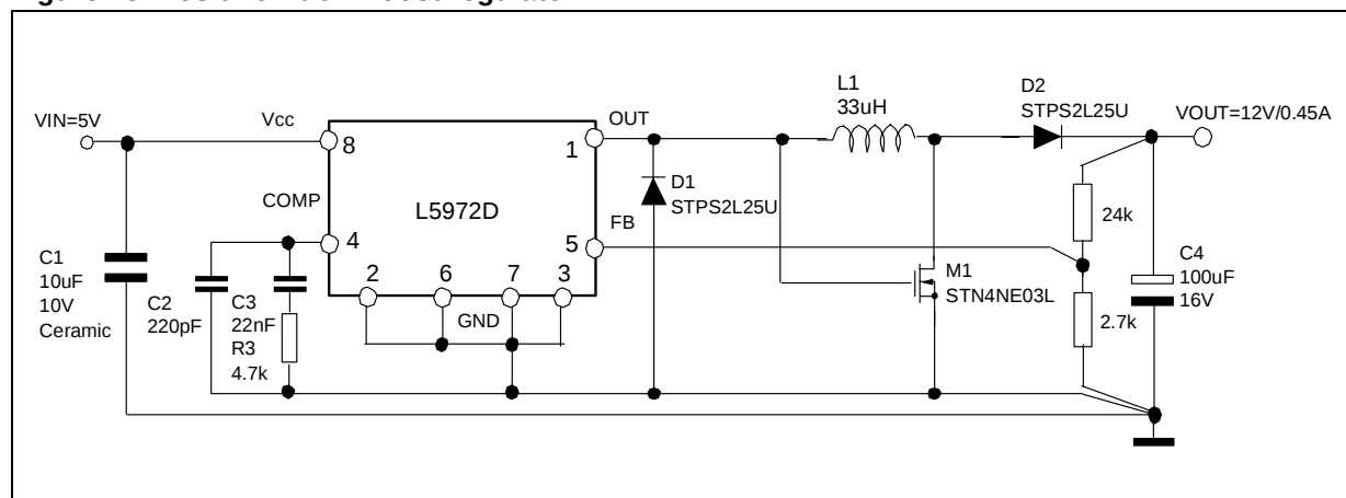
Figure 16. Buck-Boost regulator
