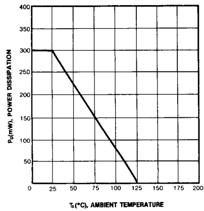
POWER DERATING
