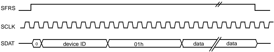
Figure 26. A Typical 3-wire Write to Data Register
