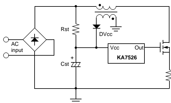
Fig.1.1 Start-up Circuit
