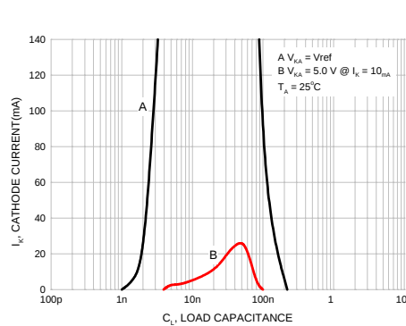
Figure 10. Stability Boundary Conditions
