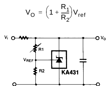
Figure 11. Shunt Regulator
